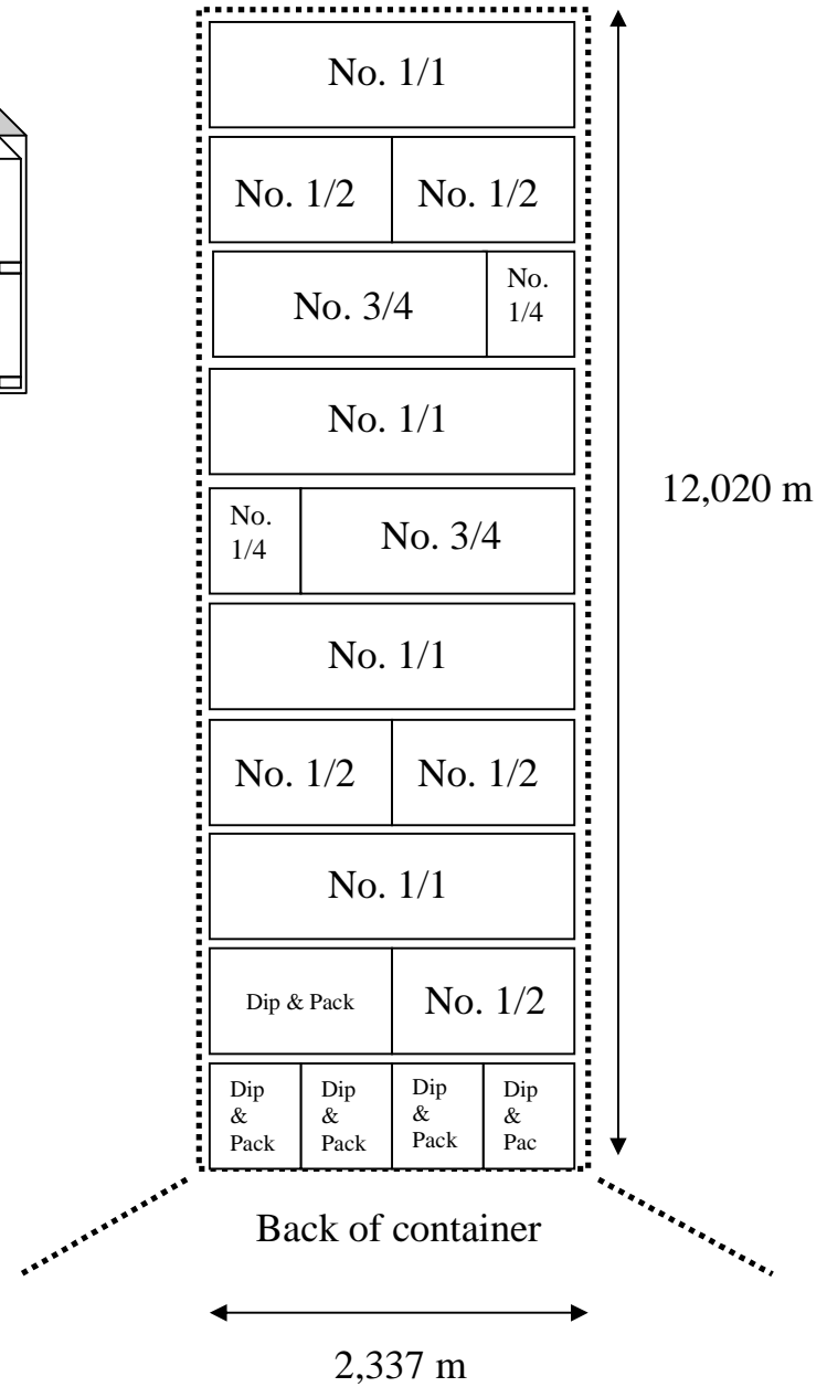
40' High Cube
